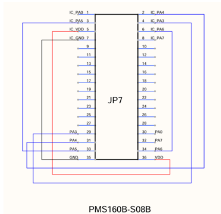
Fig. 29: schematic diagram of PMS160B-S08B Jumper7 when using P-003B
