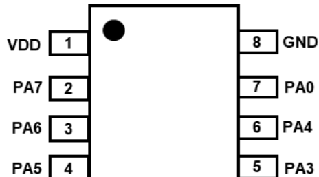
PMS160B-S08A: SOP8 (150mil)
