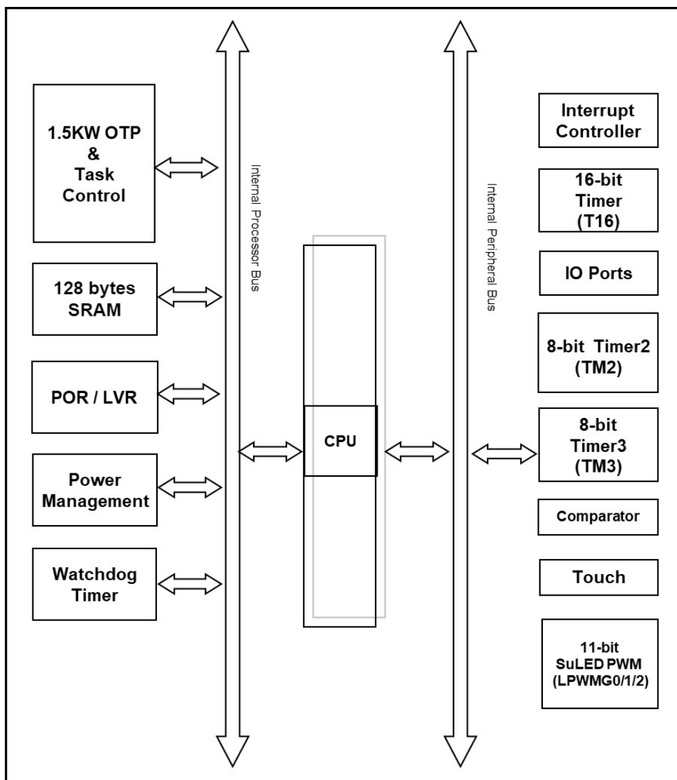
Fig. 1: PMS160B Block Diagram
